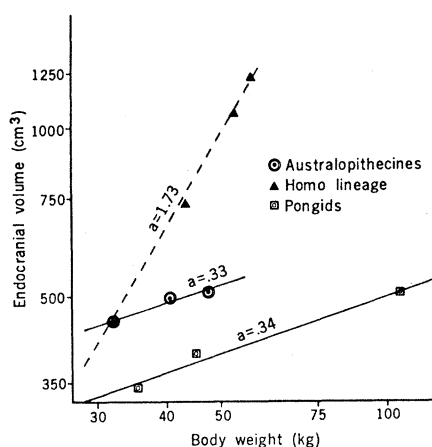
Fig. 2. Scaling of endocranial volume in pongids and hominids. We believe that estimates for hominid body weights are accurate within about 20 percent. The criterion for intraspecific functional equivalence is a = 0.2 to 0.4 .
